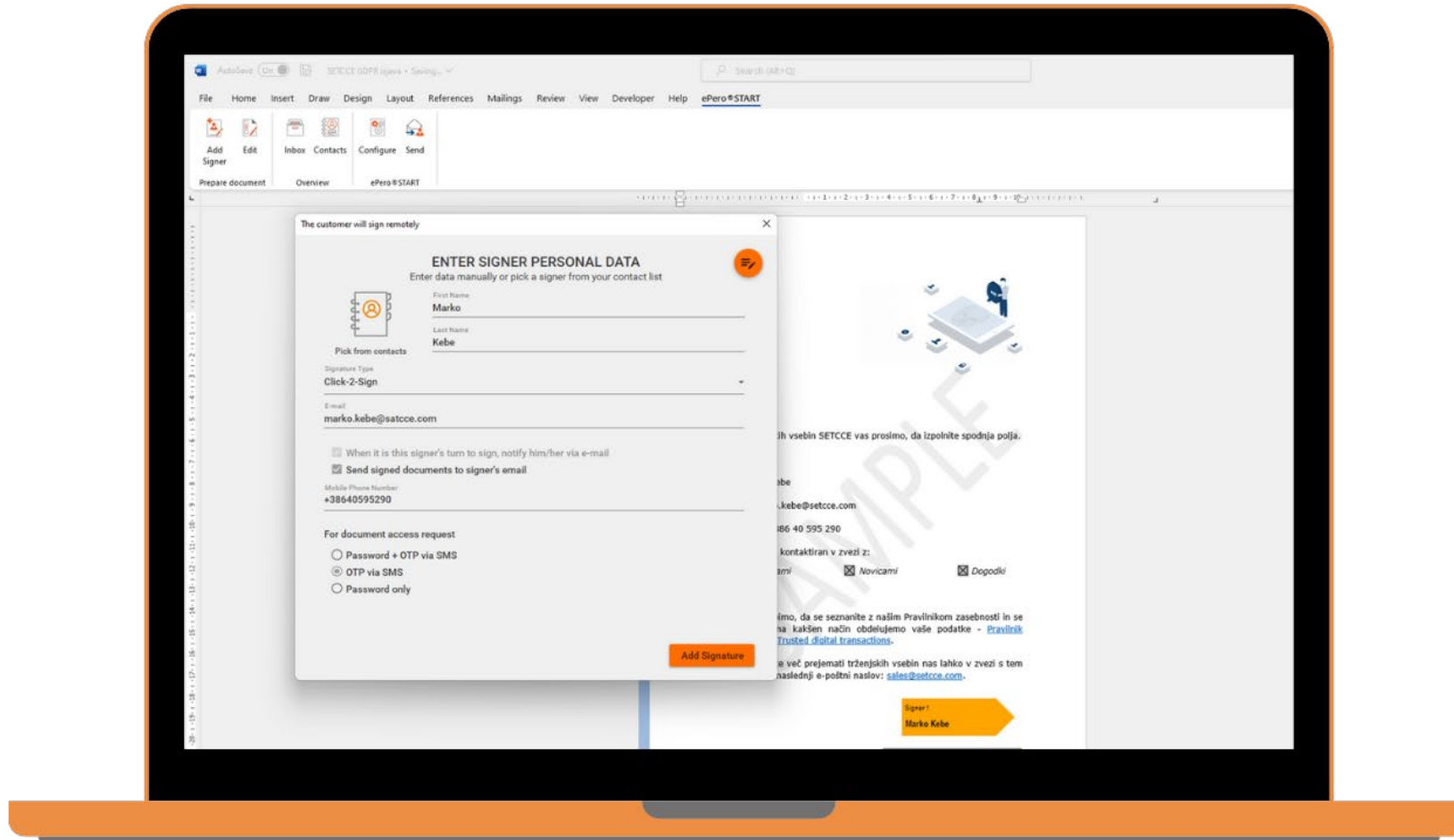
Word Add-in
